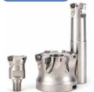
MFH Harrier ø25-ø160
